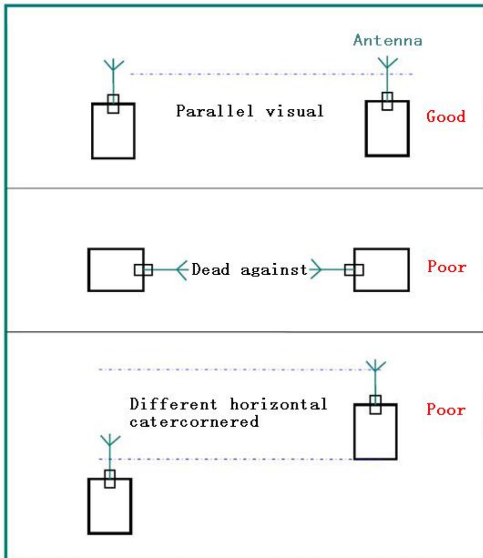
Figure 2-2 Installation antenna mode
